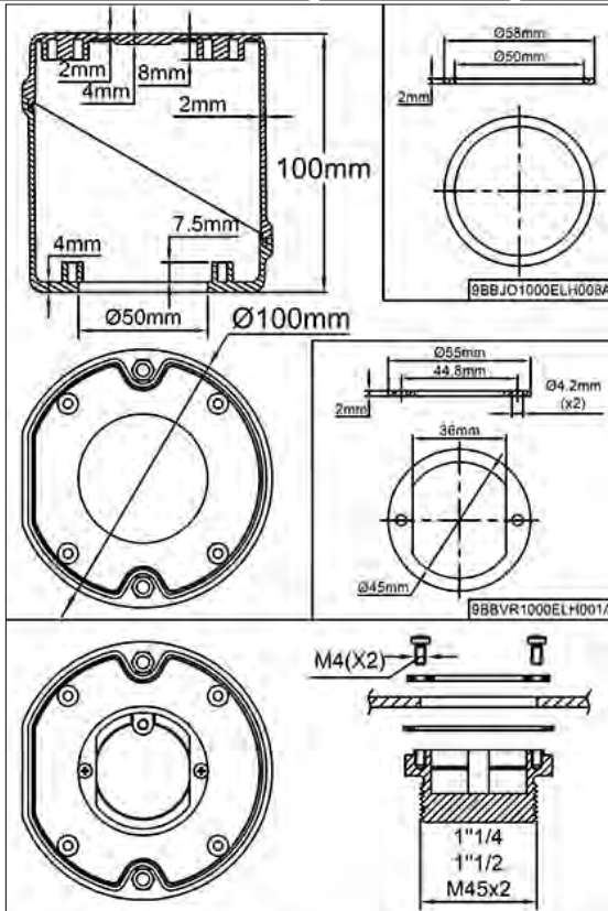
Mobile brass fitting with 2 hole ring*
